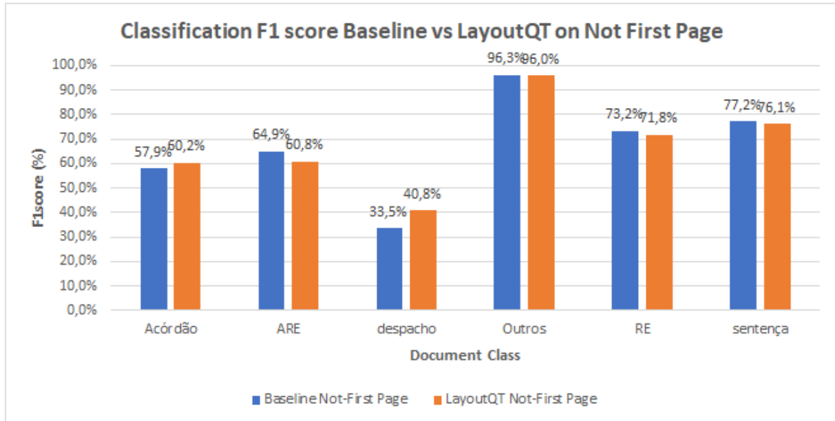
Figure 4.13: F1 score (in %) of document image classification using baseline and LayoutQT using AWD-LSTM architecture on the VICTOR Not First page sample dataset.
