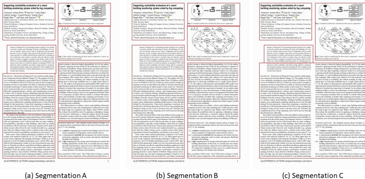
Figure 2.3: An example image showing different segmentations of the same document. Segmentations A and B are both correct as they separate text in different columns as well as images from text. Segmentation C is considered to have two errors: 1) text in the first two columns is merged 2) Caption of the top figure is merged with the figure itself.
