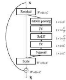
(e) SENet
